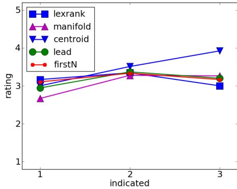
Figure 1: Graph of indicated vs. user rating for the different summarisation algorithms
