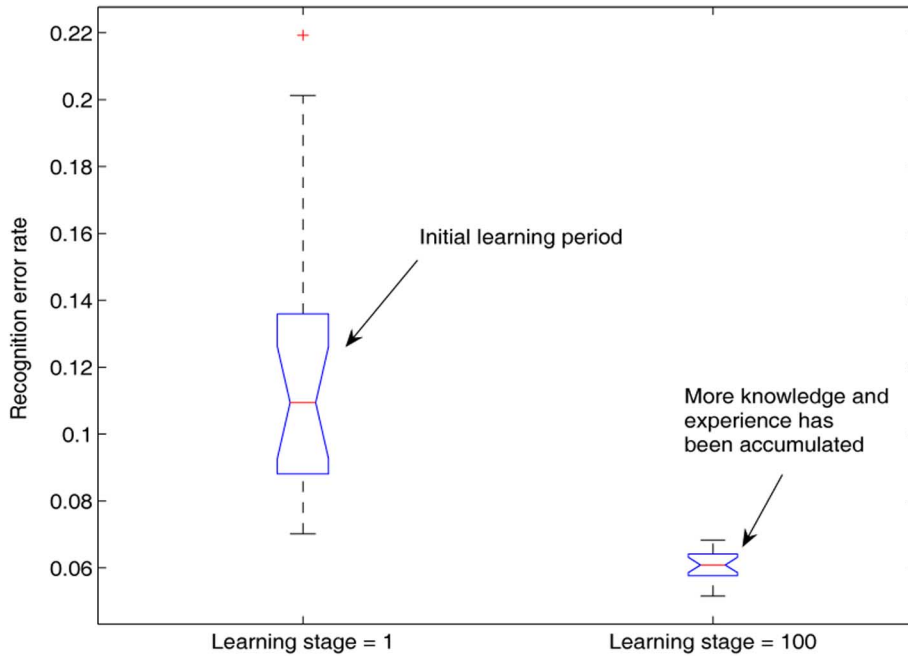
Fig. 8. Visualization of testing error statistics during different learning stages.
