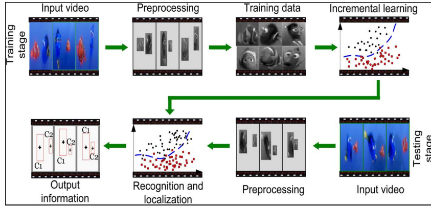
Fig. 2. IMORL framework for video data analysis.
