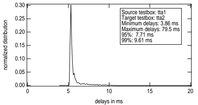
Fig. 2. A class A typical end-to-end distribution
