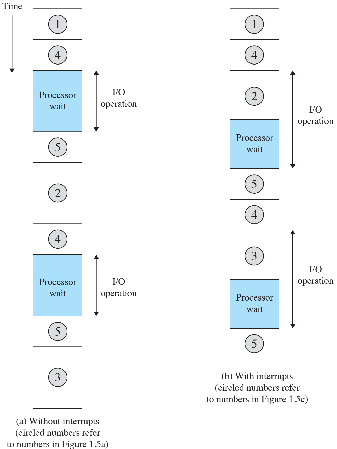
Figure 1.9 Program Timing: Long I/O Wait
