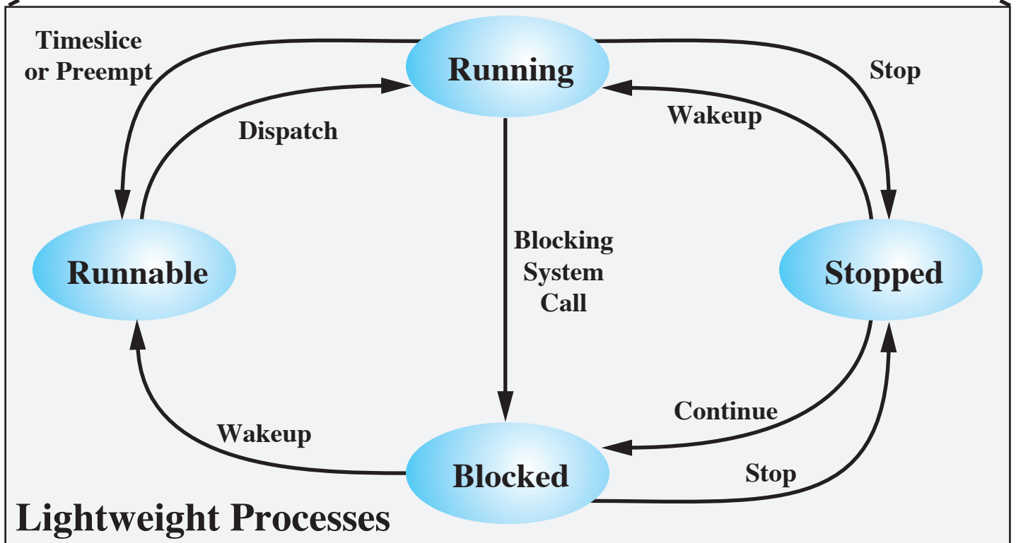
Figure 4.19 Solaris User-Level Thread and LWP States
